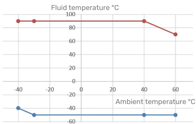
Operating temperature range for close coupled RHE45
