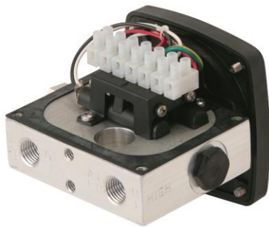
Model 124 Terminal Switch exposed.
